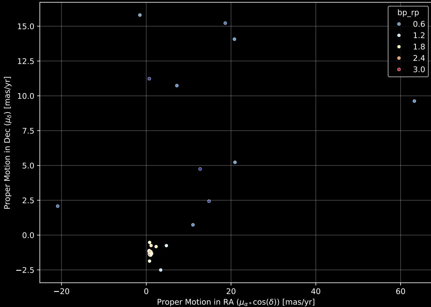
APOGEE DR17 Field: [300-44-O] Proper Motion Diagram (n= 70)
