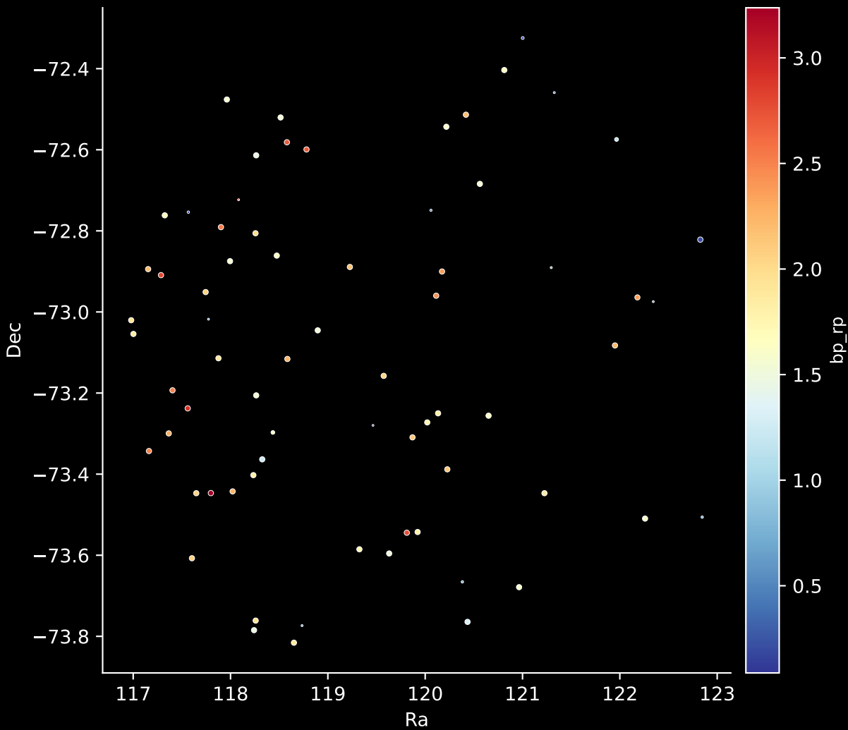
APOGEE DR17 Field: [300-44-O] Stars: 70
