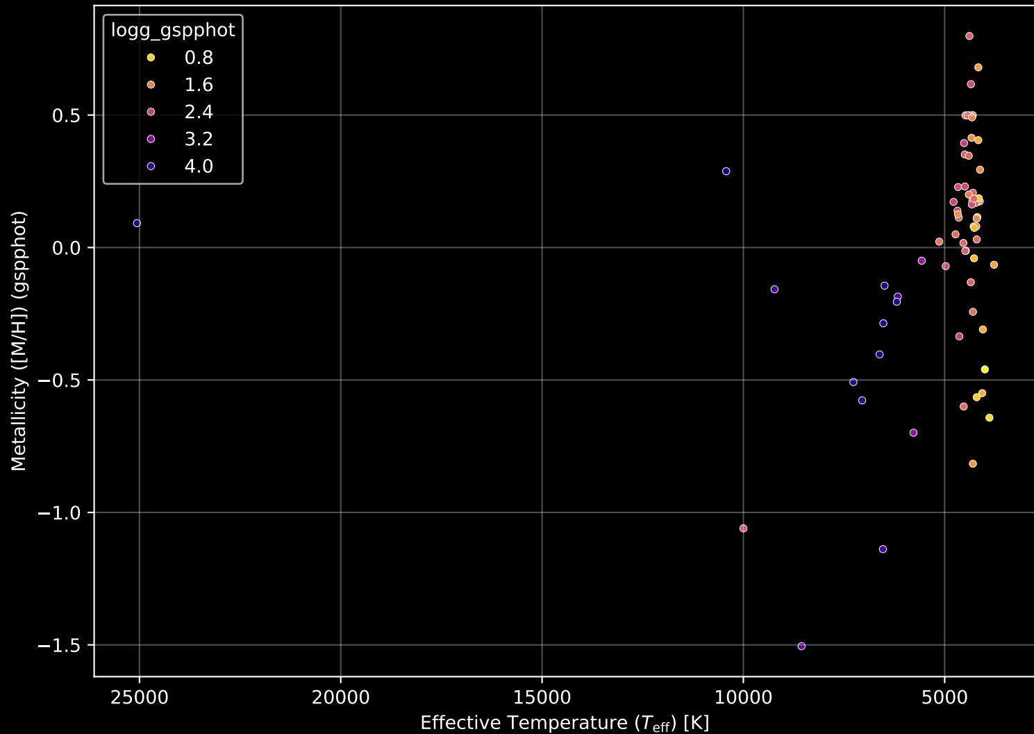
APOGEE DR17 Field: [300-44-O] Stellar Population Parameters (n= 70)
