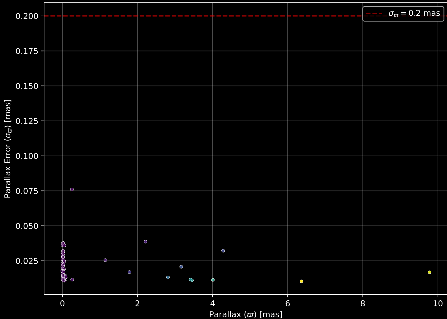
APOGEE DR17 Field: [300-44-O] Parallax Quality (n= 70)
