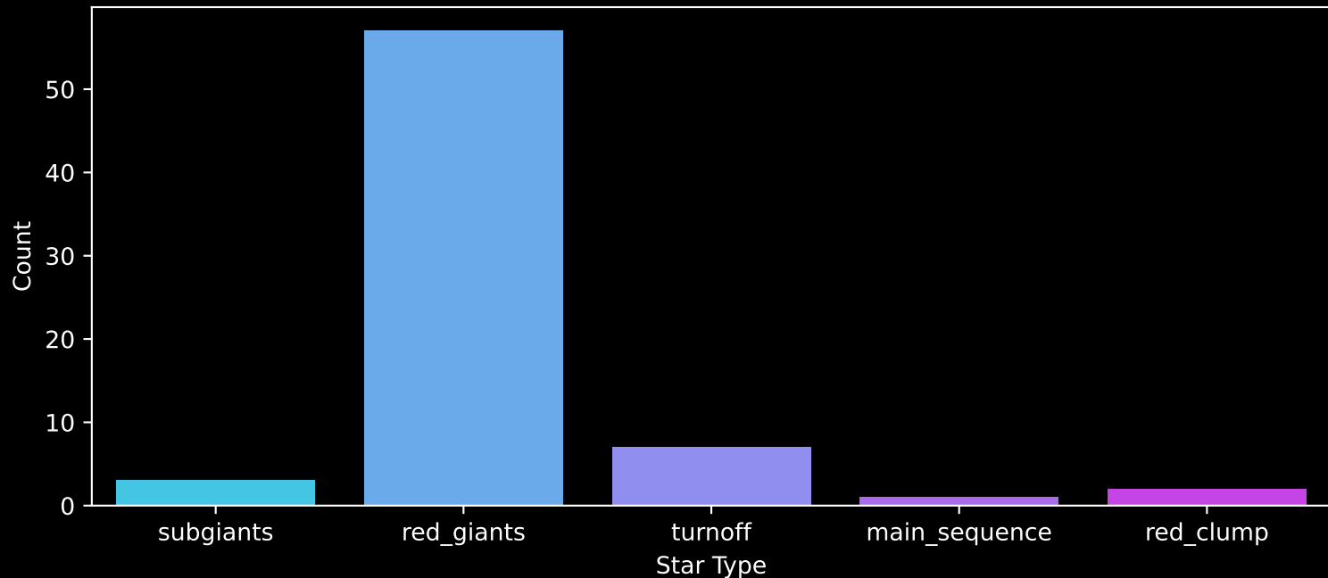
APOGEE DR17 Field: [300-44-O] Count plot of Star Type
