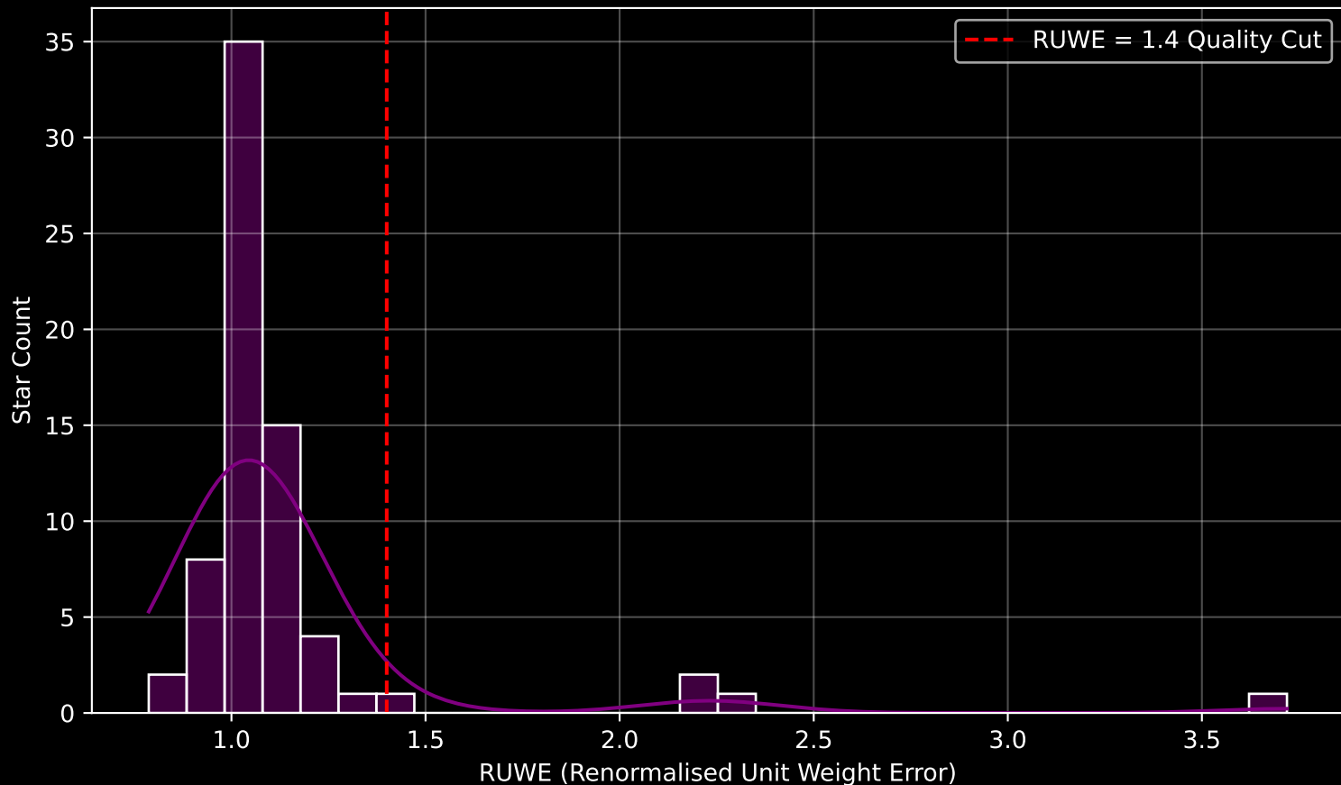
GAPOGEE DR17 Field [300-44-O] RUWE Distribution (n= 70)
