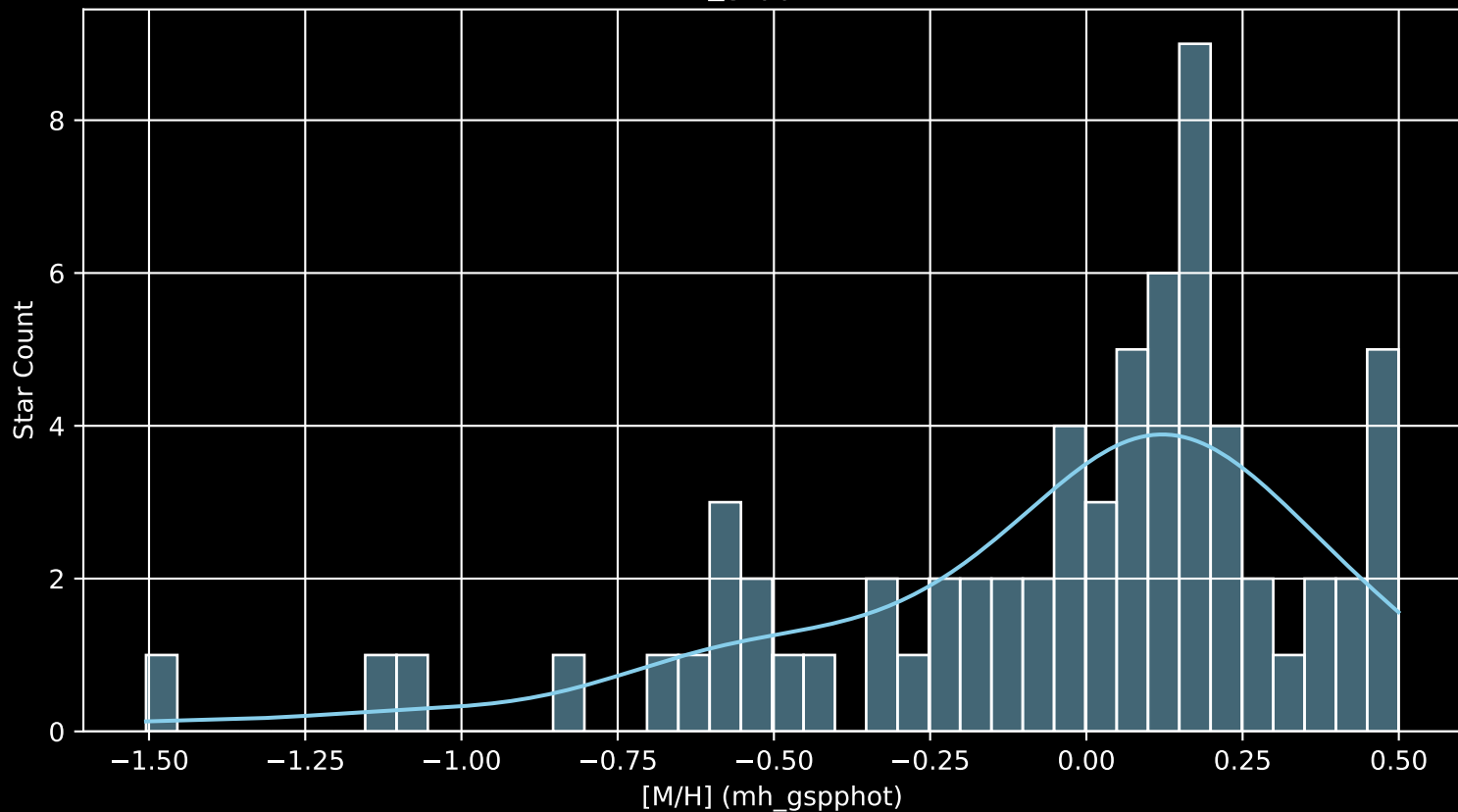
APOGEE DR17 Field: [300-44-O [M/H] (mh_gspphot) (n= 67)
